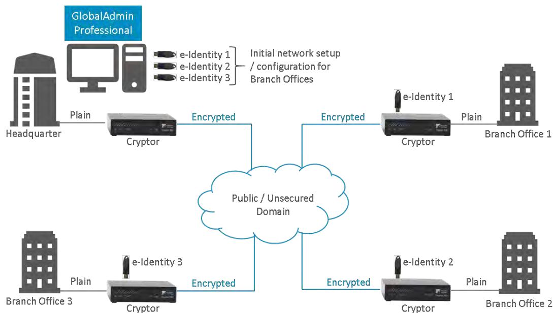
Figure 1 - Typical Company's Network
