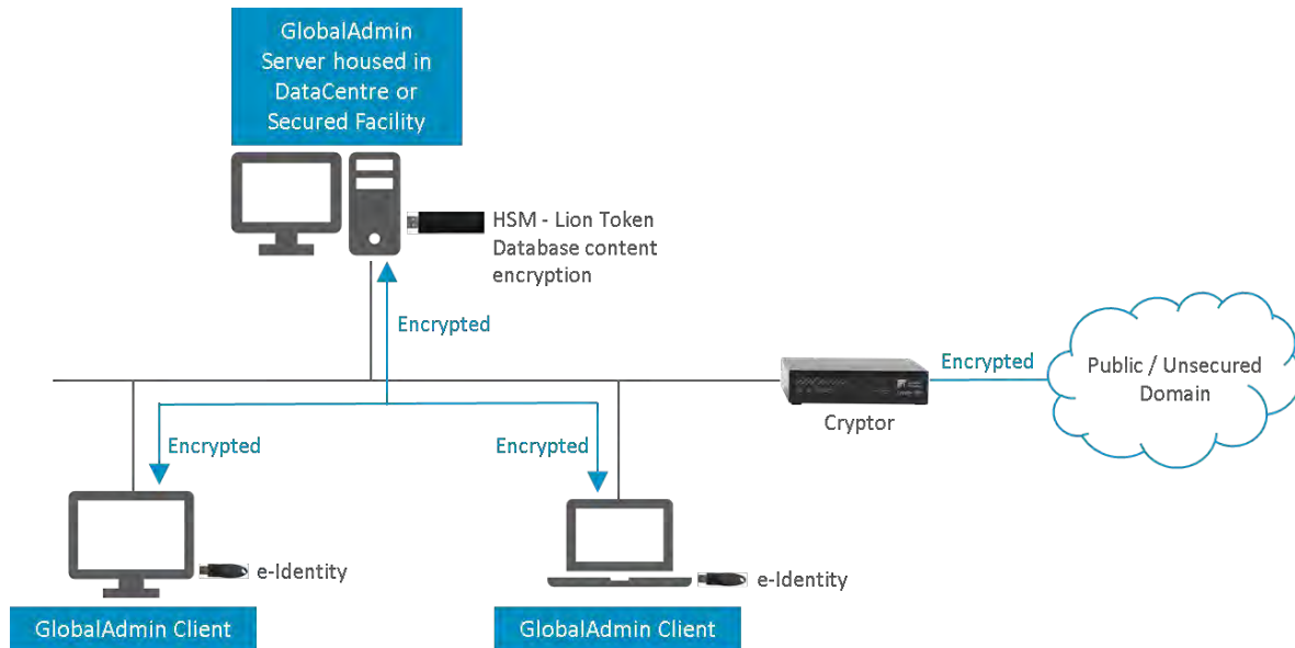
Figure 2 - Server-Client Network
